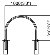
In-Situ Stainless
