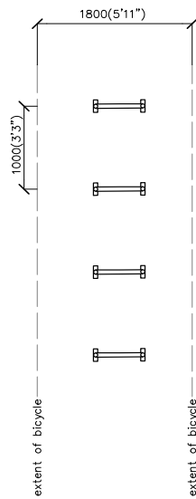
Plastic/Galvanised layout
